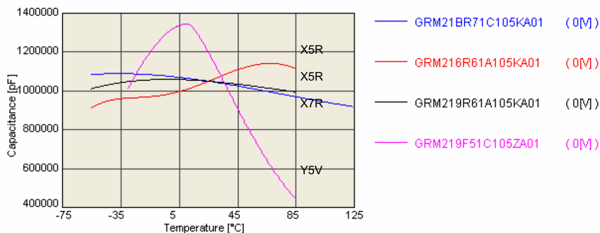
Figure 3 Ceramic Capacitance vs. Temperature
